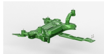
Front_Suspension_Support
