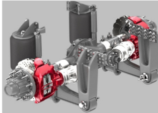
Rear_Suspension_and_Breaks
