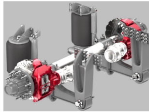
Middle_Suspension_and_Breaks
