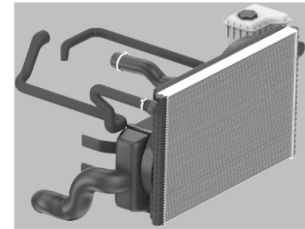
Cooling_and_Climate
