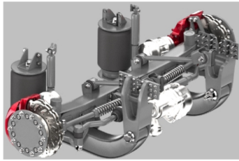
Front_Suspension_and_Breaks
