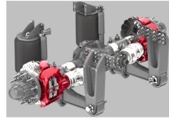
Rear_Suspension_and_Breaks
