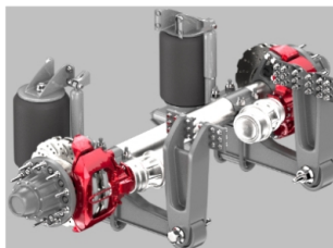
Middle_Suspension_and_Breaks
