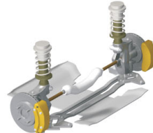
FrontSuspension4.psd
