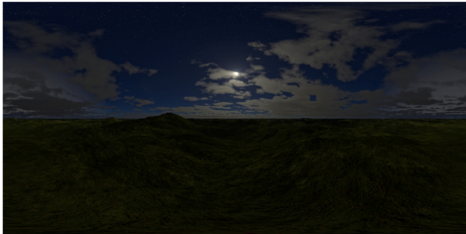
NightSky19
