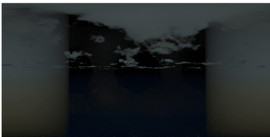
NightSky09
