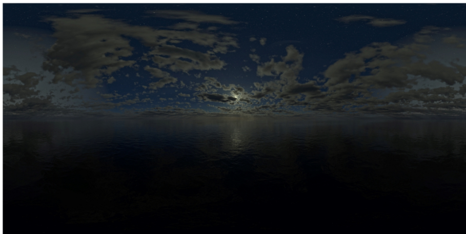
NightSky18
