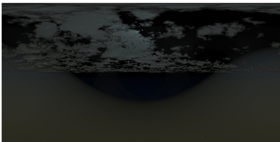
NightSky08
