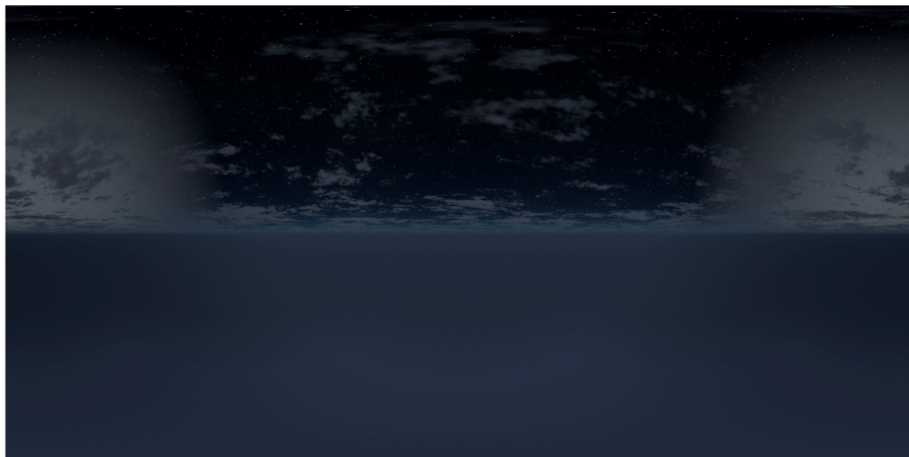
NightSky14
