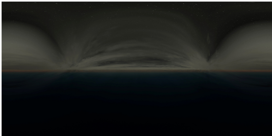
NightSky17
