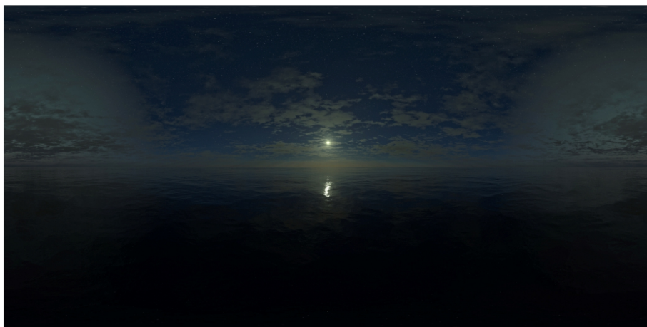
NightSky20
