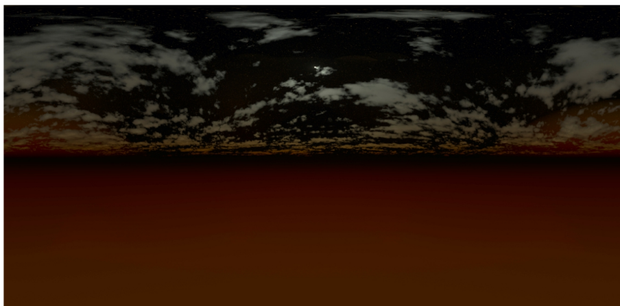
NightSky07
