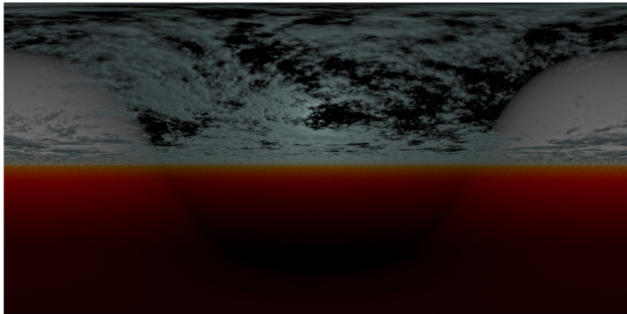
NightSky04
