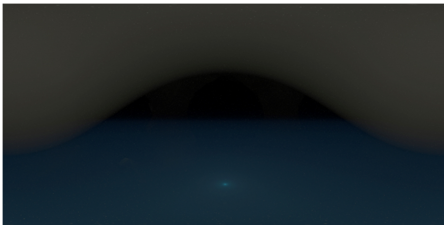
NightSky05
