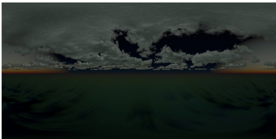
NightSky03
